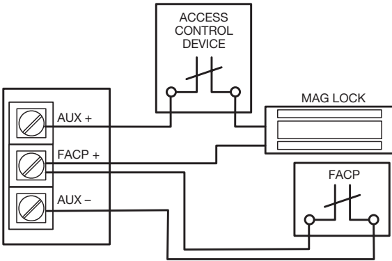
Fig. 5 - Latching fire alarm tie-in with manual reset:
